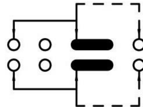
SCHEMATIC (NON-SHORTING)
